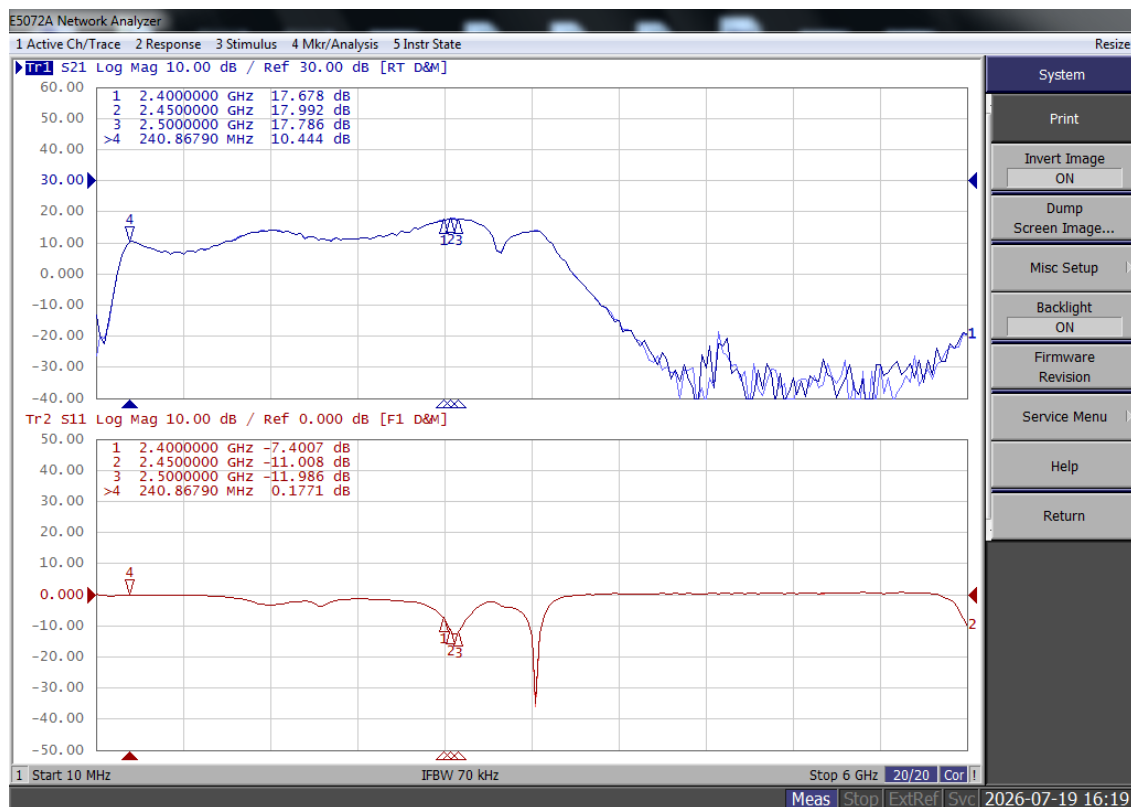
Figure 2: S11/S21 output from Network analyser
