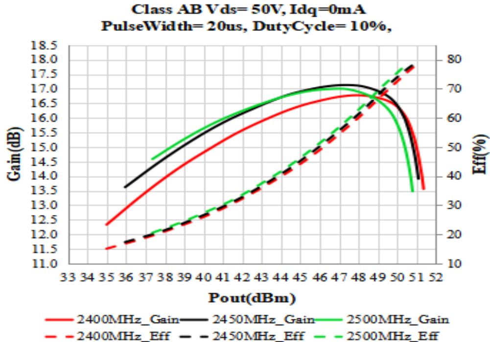
Figure 1: Efficiency and power gain as function of Pout
